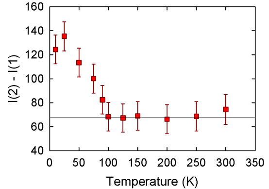
FIG. 4. Temperature dependence of the difference in the neutron scattering intensity at \mathbf{q} = (3.25, 0, 0) between the energy range 1 (51 - 55 meV) and range 2 (56 - 68 meV). The plot shows I(1) - I(2) , determined by the triple-axis spectrometer. The superconducting transition temperature of this sample is 93 K; the data show a striking resemblance to the temperature dependence of the superconducting order parameter.
